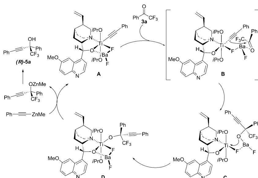
Scheme 1. Proposed mechanism and transition-state models for the alkylation of 3a into 5a .
