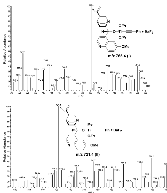
Figure 1. ESI-MS experiment of the intermediates ( I ) and ( II ).
